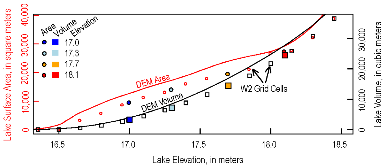
Figure 3. Graph showing comparison of water-surface elevation, lake surface area, and lake volume from CE-QUAL-W2 grid and a digital elevation model (DEM) for Crystal Springs Lake, Portland, Oregon.
