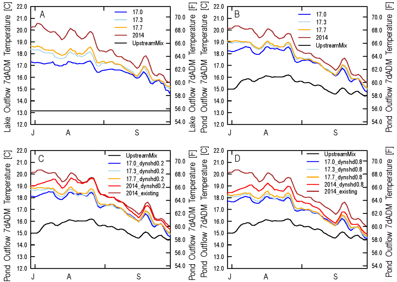
Figure 12. Graphs showing comparison of the 7-day average of the daily average maximum temperatures (7dADM) resulting from different lake surface elevation scenarios. Results shown for (A) total weighted average of outflow from Crystal Springs Lake (sites Spill and FL) using 2014 shading of Crystal Springs Lake, (B) outflow from the Golf Pond (site CSDS) using 2014 shading of Crystal Spring Lake, (C) outflow from the Golf Pond (site CSDS) using 20 percent shading of Crystal Spring Lake, and (D) outflow from the Golf Pond (site CSDS) using 80 percent lake shade of Crystal Spring Lake.
