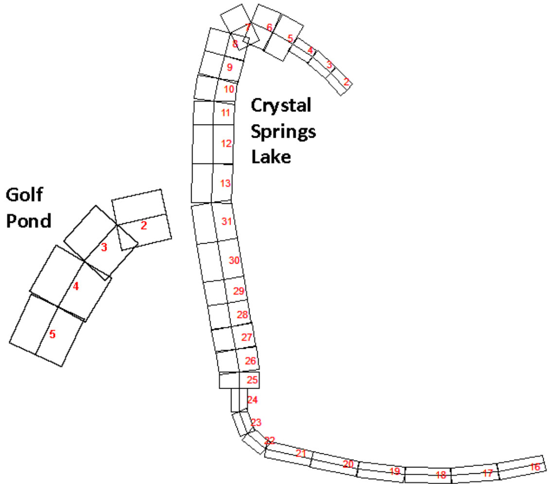
Figure 5. Diagram showing CE-QUAL-W2 model grid of Crystal Springs Lake and the Golf Pond, Portland, Oregon.
