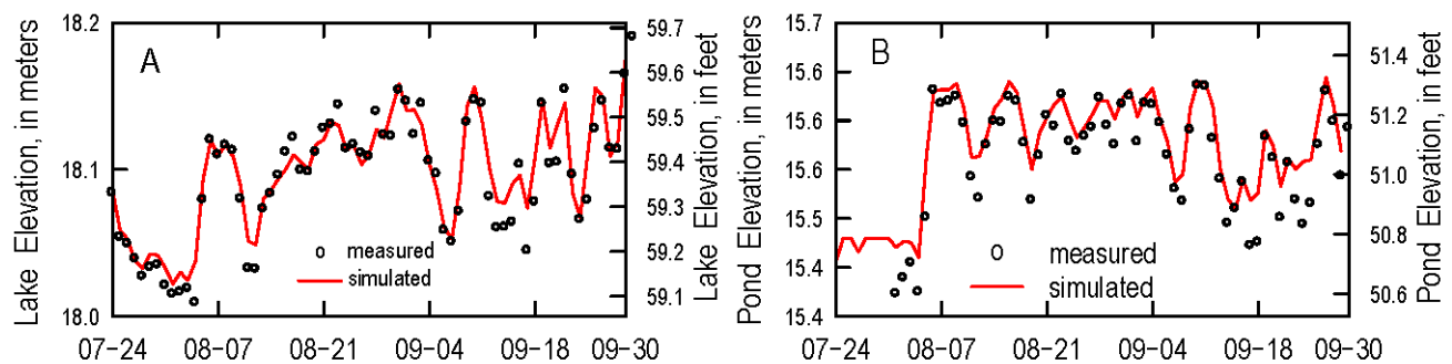
Figure 7. Graphs showing measured and simulated water surface elevation of (A) Crystal Springs Lake and (B) the Golf Pond, Portland, Oregon.
