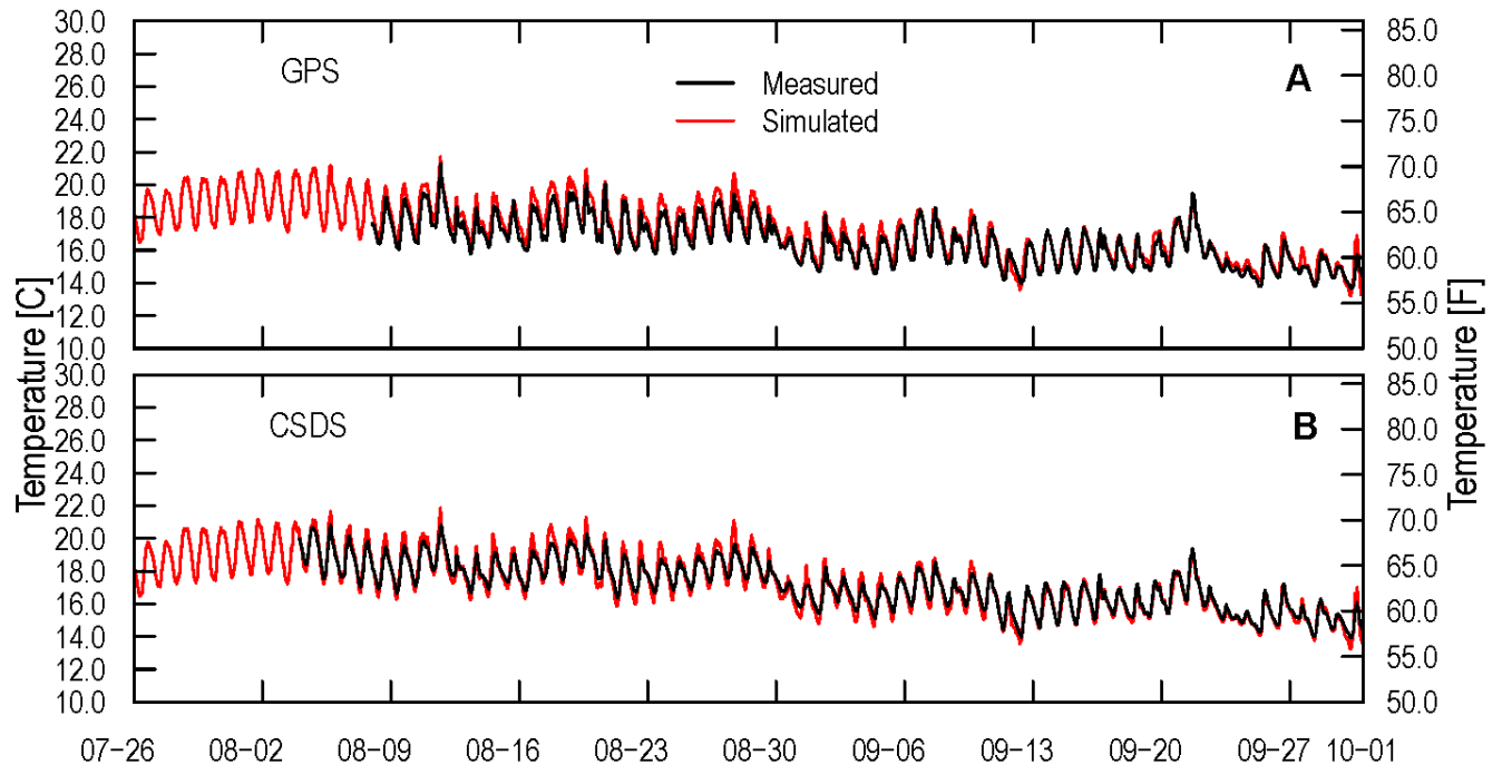
Figure 11. Graphs showing comparison of measured and simulated temperature at sites (A) east arm of the Golf Pond (GPS) and (B) Crystal Springs Creek above railroad (CSDS), Crystal Springs Lake, Portland, Oregon.
