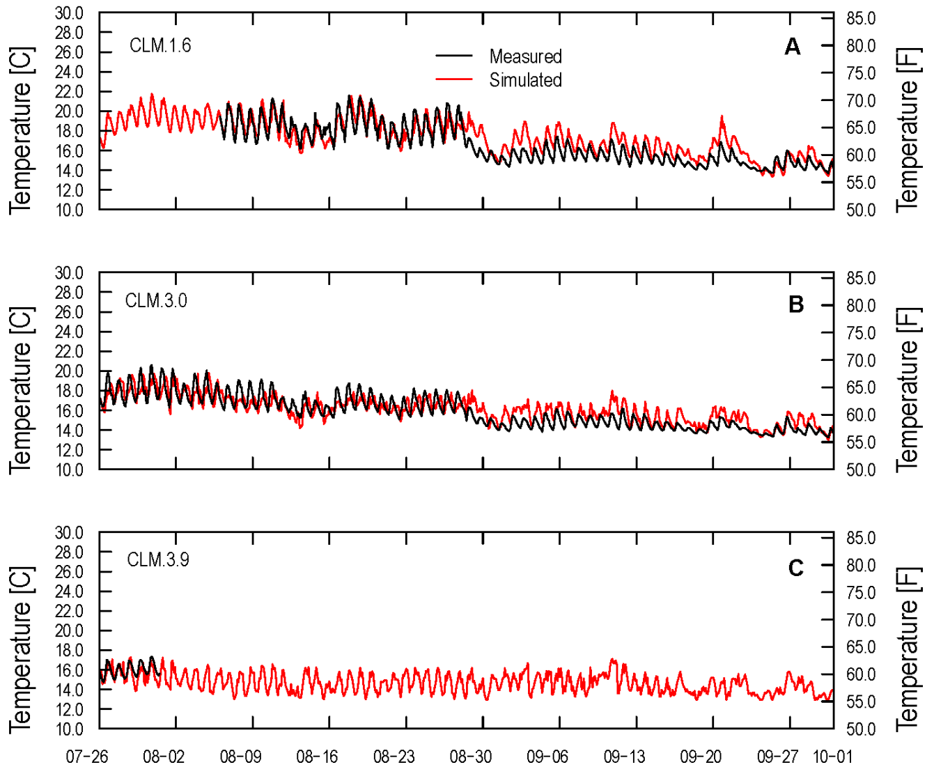
Figure 10. Graphs showing comparison of measured and simulated water temperature at sites (A) Crystal Springs Lake Middle (depth = 1.6 ft; CLM.1.6); (B) Crystal Springs Lake Middle (depth = 3.0 ft; CLM.3.0); (C) Crystal Springs Lake Middle (depth = 3.9 ft; CLM.3.9).
