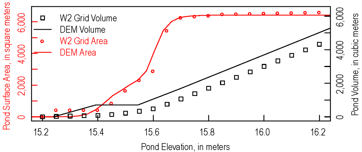
Figure 4. Graph showing comparison of water-surface elevation, surface area, and volume from CE-QUAL-W2 grid and a digital elevation model (DEM) for the Golf Pond, Portland, Oregon.
