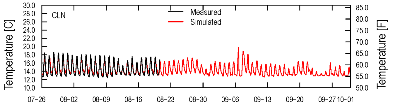
Figure 8. Graph showing comparison of measured and simulated water temperature at site Crystal Springs Lake North (CLN), Crystal Springs Lake, Portland, Oregon.
