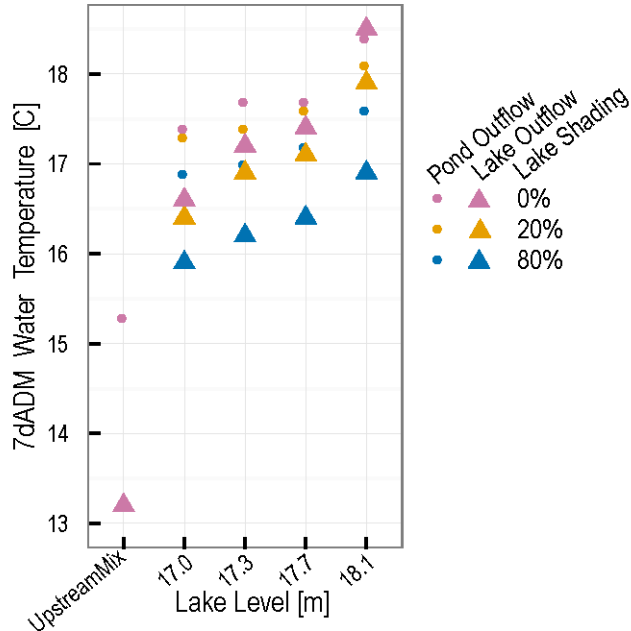
Figure 13. Graph showing comparison of 2-month simulation period of average 7-day moving average of daily maximum temperature under various scenarios downstream of Crystal Springs Lake (triangles) and the Golf Pond (circles), Portland, Oregon.
